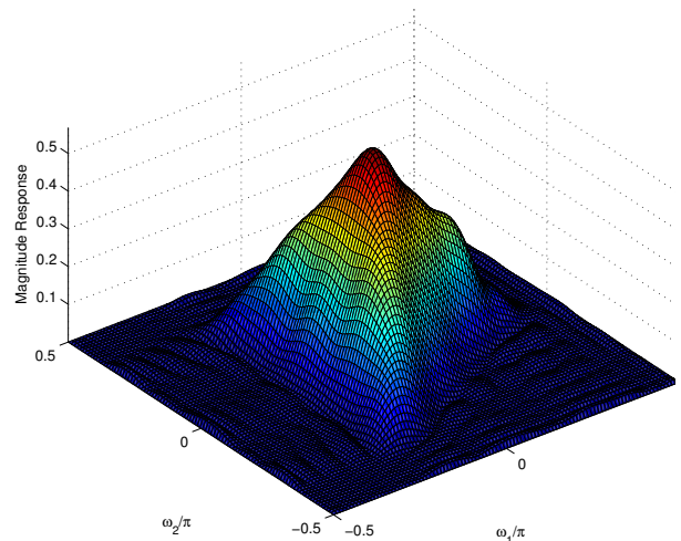
Fig. 2. Magnitude frequency response of 15 \times 15 two-dimensional filter.
