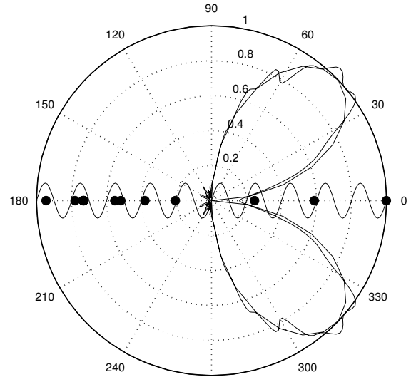
Fig. 1. Magnitude beamforming with arbitrary array geometry. The array element locations are shown as small circles along with a wave (indicating relative wavelength).
