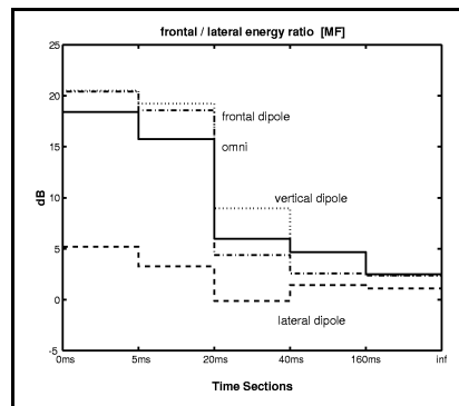
Figure 8b. Time evolution of the ratio between frontal (cardio mic.) and lateral (bi-directional mic.) energy
