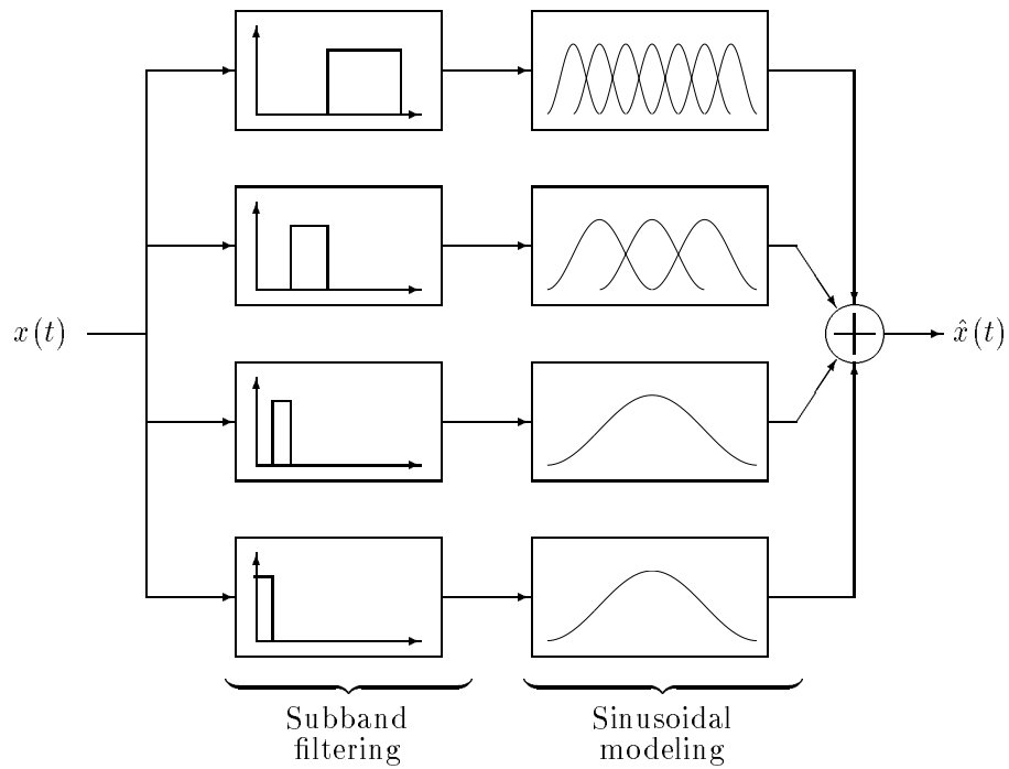
FIGURE 3.9: Multiresolution sinusoidal modeling with a nonsubsampling filter bank. The filter bank in this simple depiction provides an octave-band decomposition; the sinusoidal models have frame sizes scaled by powers of two according to the width of the respective subband. As described in the text, it is straightforward to design filter banks that derive other decompositions but it is not feasible to optimize the filter bank and the sinusoidal models for modeling arbitrary signals.
