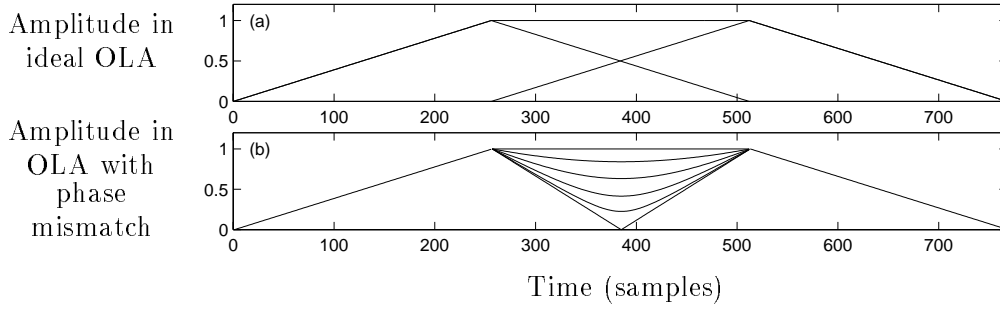
FIGURE 2.18: Plot (a) shows the ideal amplitude envelope for overlap-add with equal amplitudes in adjacent frames; the underlying triangular windows are also shown. Plot (b) shows examples of the amplitude distortion that occurs in the overlap region due to phase mismatch; this example is specifically for the case of frequencies that are equal in adjacent frames as formulated in Equation (2.105), but the effect is general as discussed in the text. In the plot, the phase mismatch \omega_1 L ranges from 0 to \pi ; for a mismatch of \pi , the signals cancel exactly at n = 3L/4 , halfway through the overlap region.
