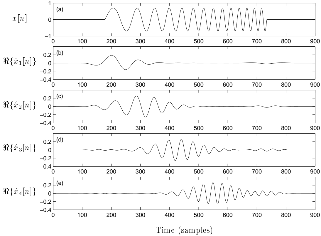
FIGURE 2.4: Reconstructed subband signals in an nonsubsampled STFT filter bank model of a chirp signal. The signals \hat{x}_k[n] correspond to those labeled in Figure 2.3 for k = \{1, 2, 3, 4\} . In the simulation, N = 128 , K = 128 , and L = 1 ; w[n] and v[n] are square-root Hanning windows.
