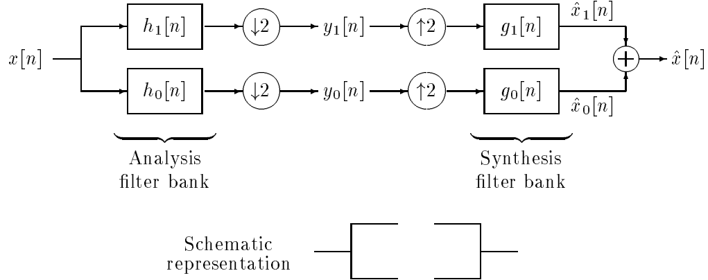
FIGURE 3.3: Critically sampled perfect reconstruction two-channel filter banks having this structure can be used to derive the discrete wavelet transform. In the literature, such a structure is often depicted with the simple line drawing shown. In many applications of such structures, h_0[n] and h_1[n] are respectively a lowpass and a highpass filter; likewise for g_0[n] and g_1[n] .
