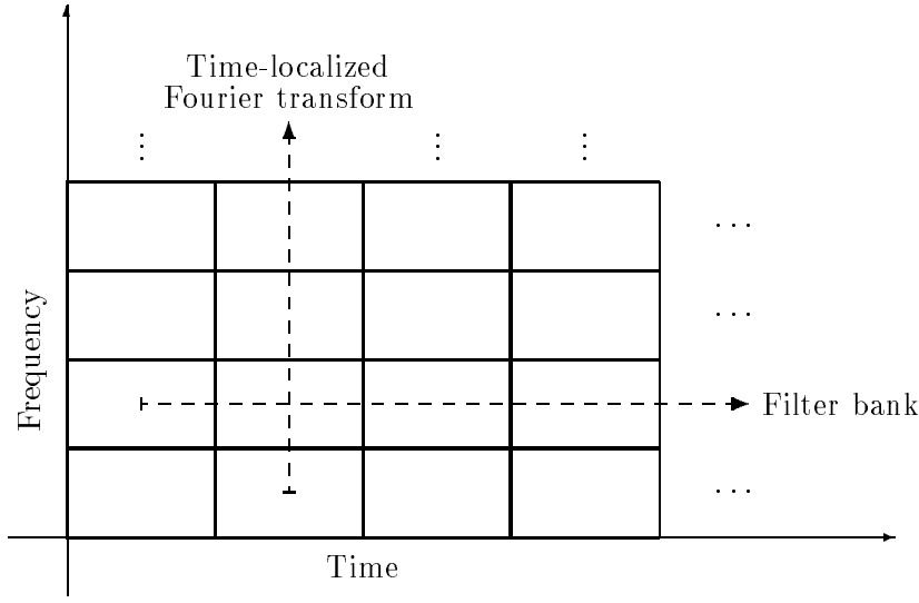
FIGURE 2.1: Interpretations of the short-time Fourier transform as a series of time-localized spectra (vertical) and as a bank of bandpass filters (horizontal).
