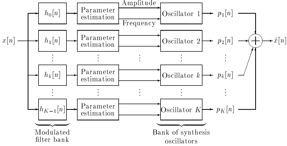
FIGURE 2.6: Block diagram of the phase vocoder. The amplitude and frequency (total phase) control functions for the K oscillators are derived from the filter bank output signals by the parameter estimation blocks.
