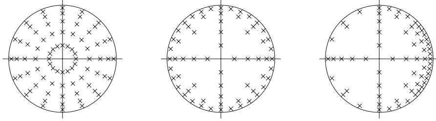
FIGURE 6.13: Filter bank interpretation and dictionary structures. The atoms in a dictionary of damped sinusoids correspond to the impulse responses of a bank of one-pole filters; for decaying causal atoms, the poles are inside the unit circle. These dictionaries can be structured in various ways as depicted above. The correlations in the pursuit are computed by the corresponding matched filters, which are time-reversed and thus have poles outside the unit circle.
