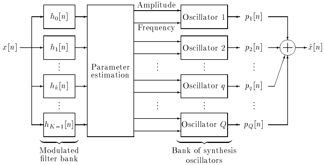
FIGURE 2.7: Block diagram of the general sinusoidal model. The amplitude and frequency (total phase) control functions are derived from the filter bank outputs by tracking spectral peaks in time as they move from band to band for an evolving signal. The parameter estimation block detects and tracks spectral peaks; unless Q is externally constrained, the number of peaks detected dictates the number of oscillators used for synthesis.
